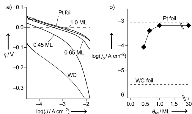
Figure 3. a) Tafel plots for WC, Pt, and sub-ML to ML Pt-WC foils in 0.5 M \text{H}_2\text{SO}_4 . Measurements were taken with a scan rate of 2\text{ mVs}^{-1} . b) Dependence of the HER exchange current density ( j_0 ) on the equivalent coverage of Pt deposited ( \theta_{Pt} ).
